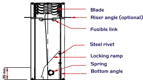
Cross sectional view single section
